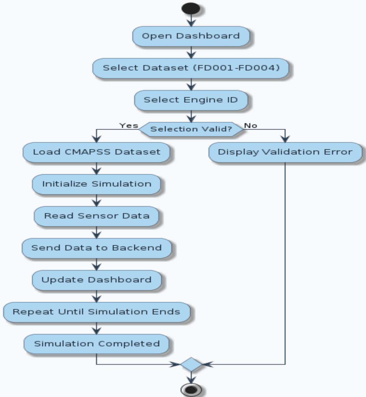
Activity Diagram - Dataset Selection & Simulation
